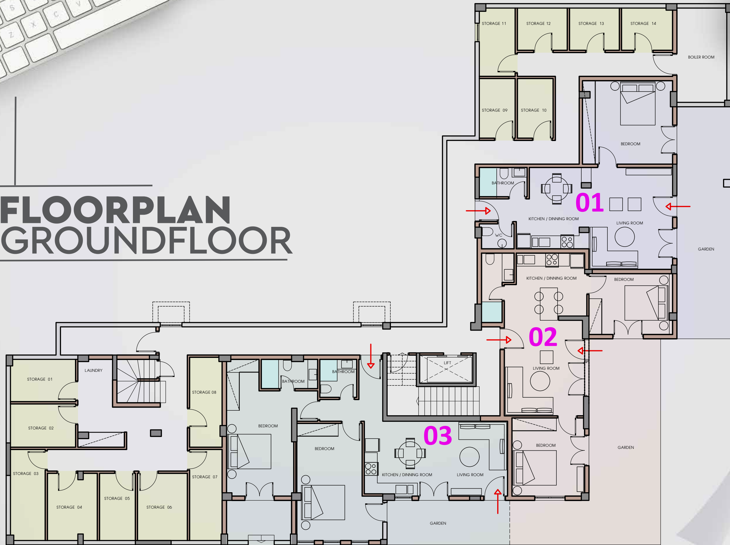
GROUND FLOOR
